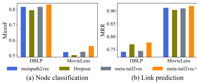
Fig. 8: Performance on head nodes w.r.t. metapath2vec as the base embedding model.
